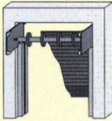
Inside Mount Under Lintel
