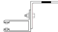
ALUMINUM EXTRUDED GUIDE
